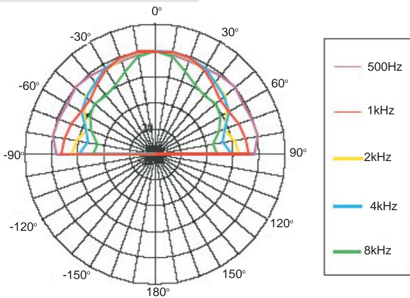
Polar pattern
