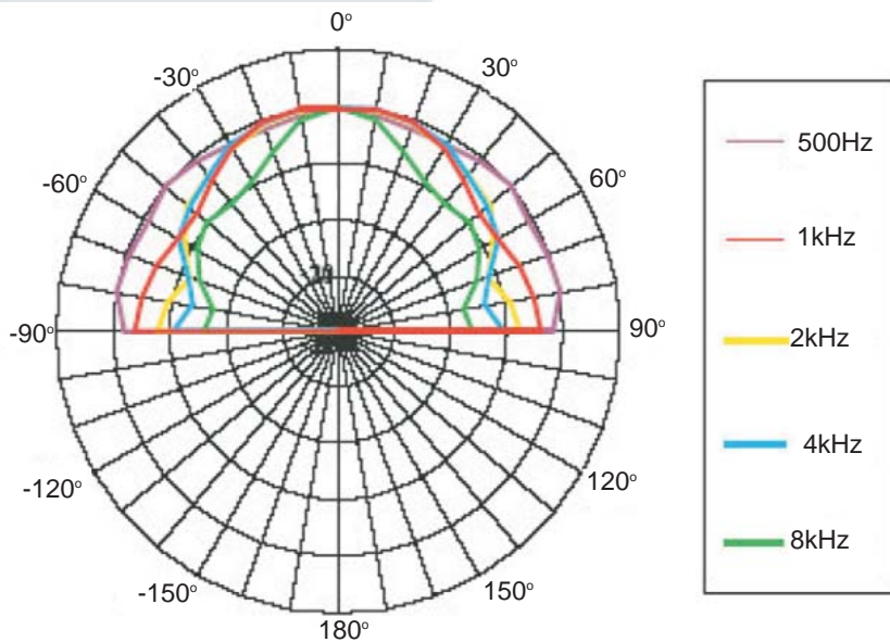
Polar pattern
