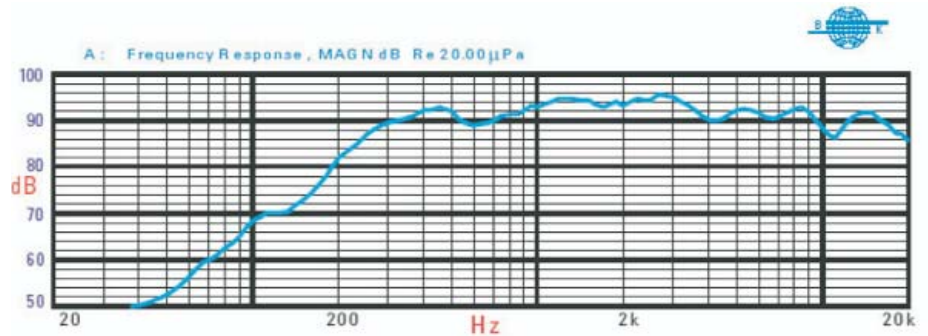
Frequency Response
