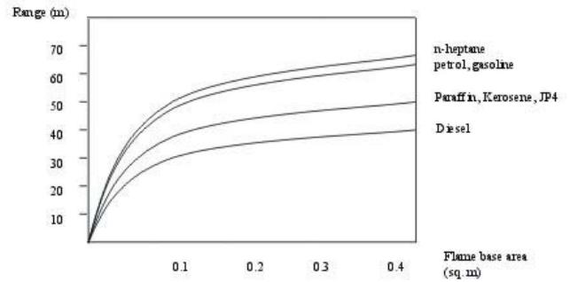
Fig. 1 - Fire Range Test Data
